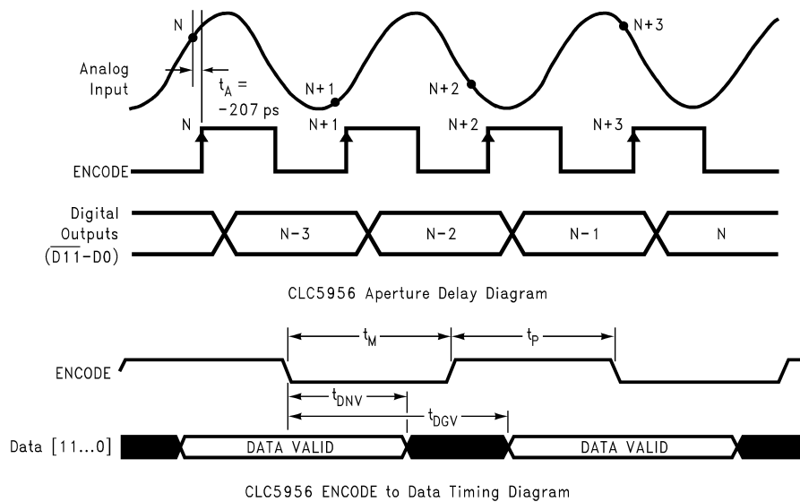
Timing Diagram
